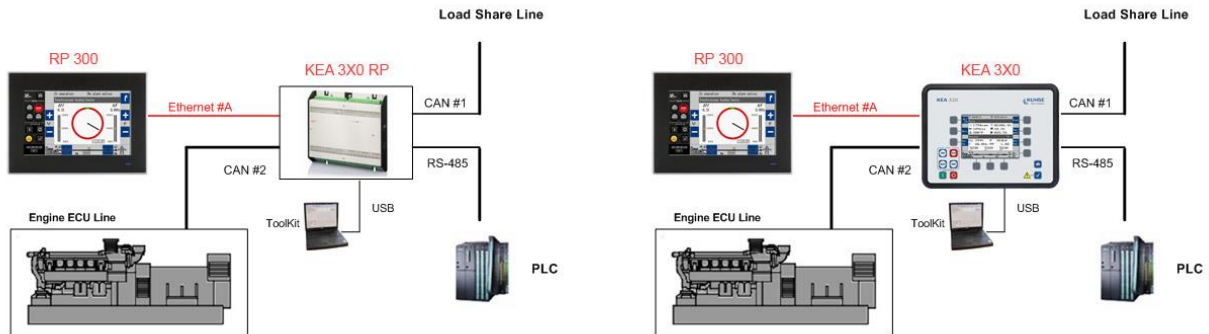
RP 300 with KEA 3X0 RP (back panel mounting)
